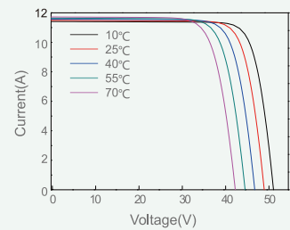
Current-Voltage Curve(SP455M-72H)
