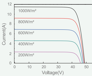
Current-Voltage Curve(SP455M-72H)
